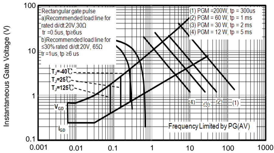
Figure6. Gate Characteristics
