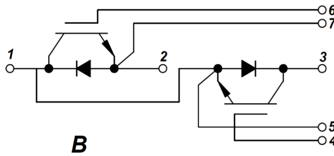
Figure 13. Circuit Diagram
