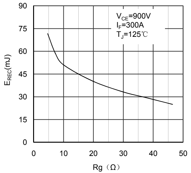
Figure 10. Switching Energy vs Gate Resistor Diode - inverter
